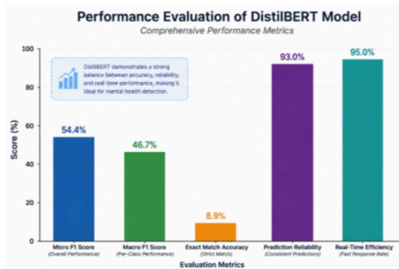
Fig 5.3: PERFORMANCE EVALUATION OF DISTILBERT MODEL
